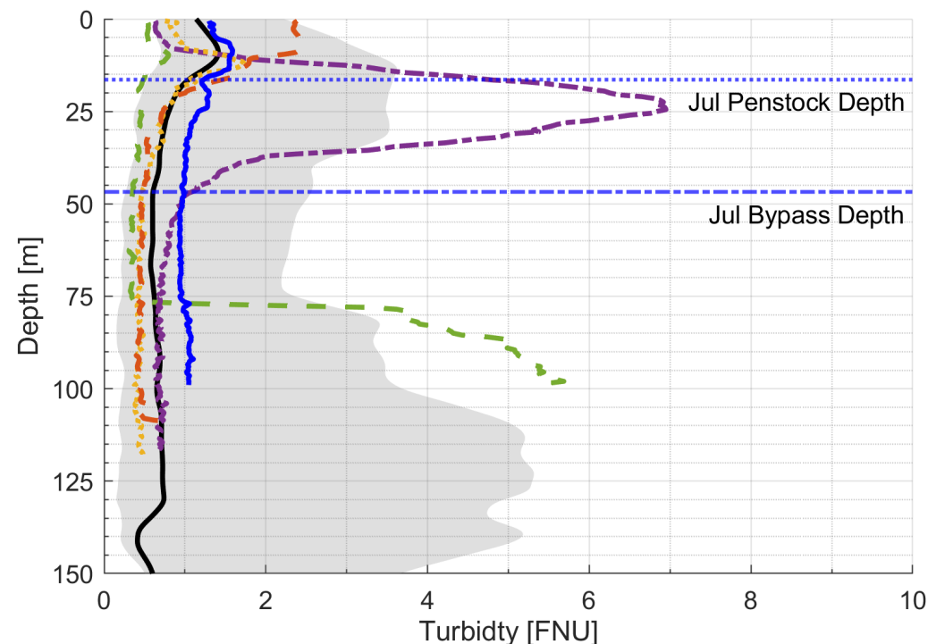
Turbidity
