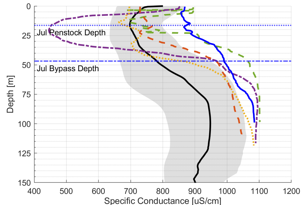
Specific Conductivity
